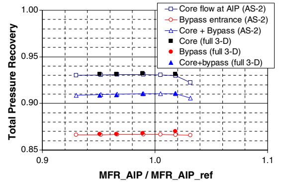
a) Total pressure recovery at AIP and bypass entrance
